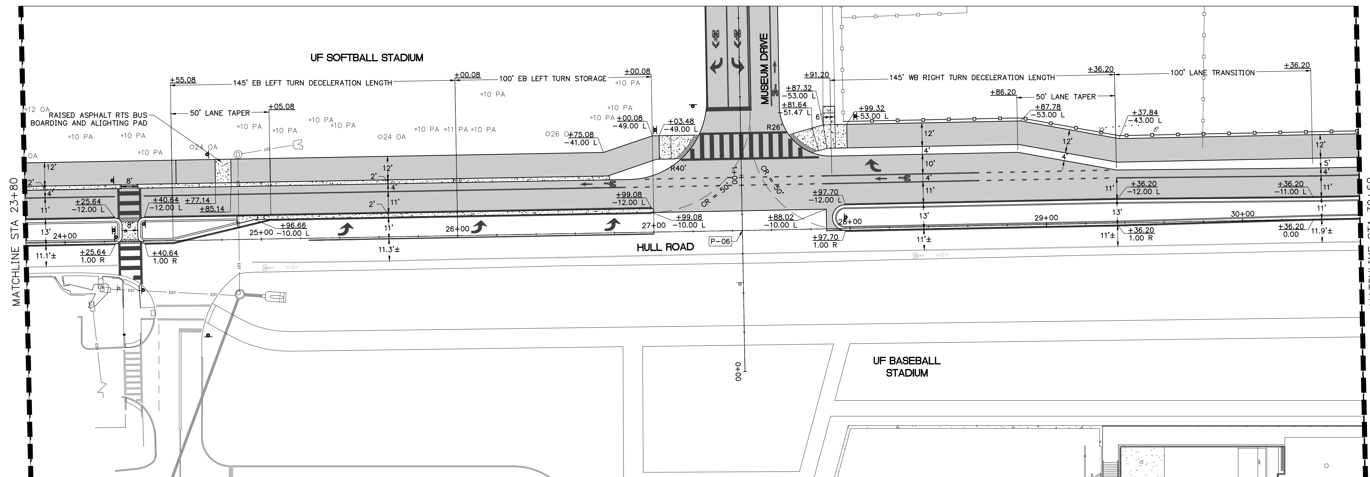
HULL ROAD - IMPROVEMENT AREA (C) STA 23+80 TO STA 30+60
